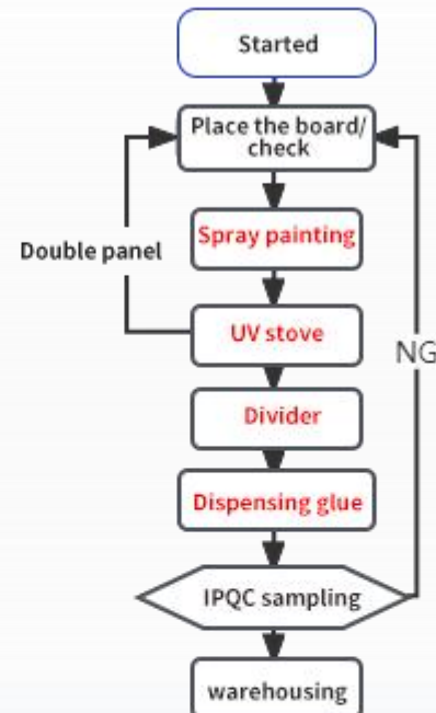
Three prevention production process flow chart
