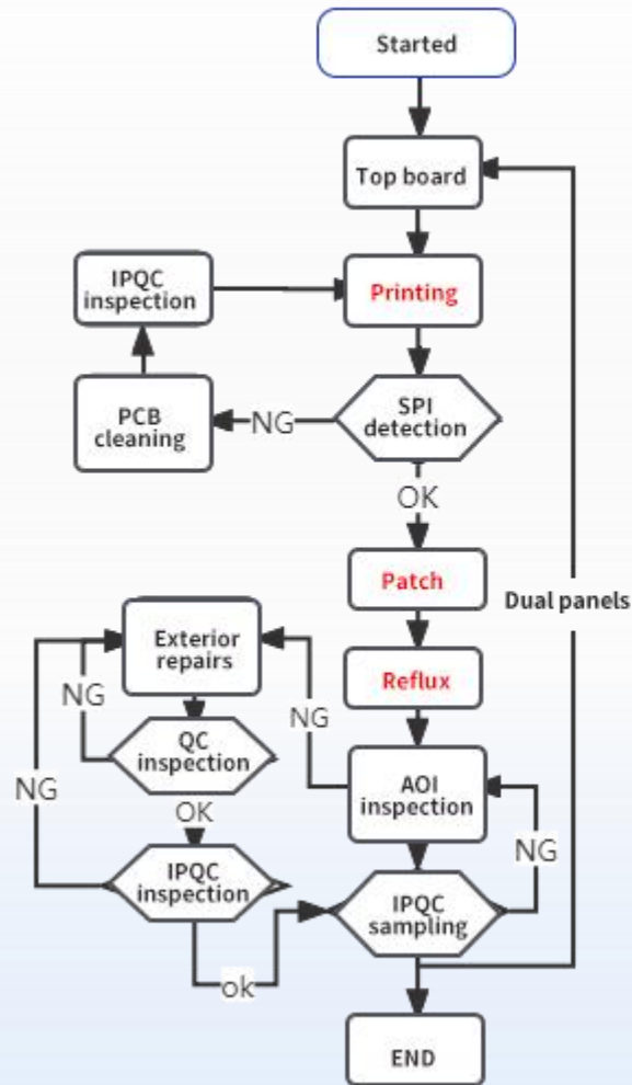
SMT production process flow chart
