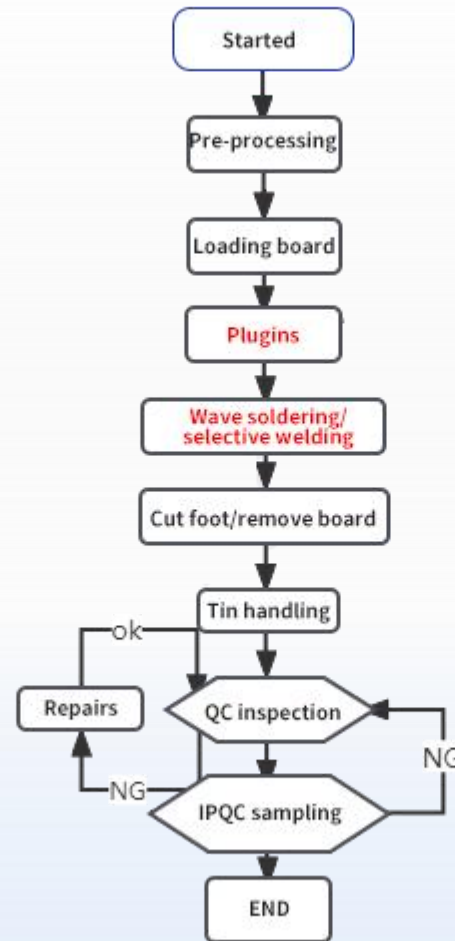
DIP production process flow chart
